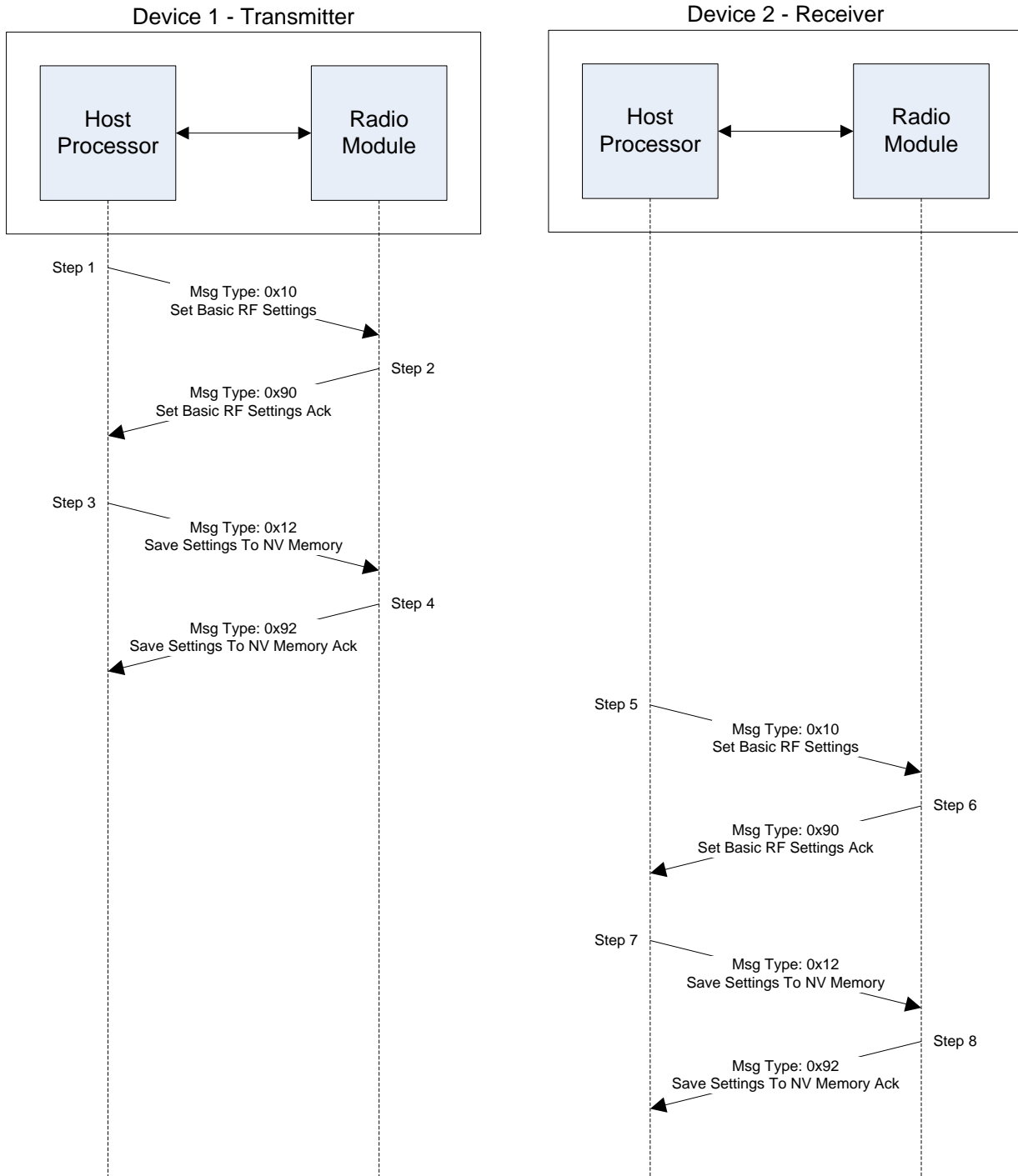
Figure 9 – Module Configuration
