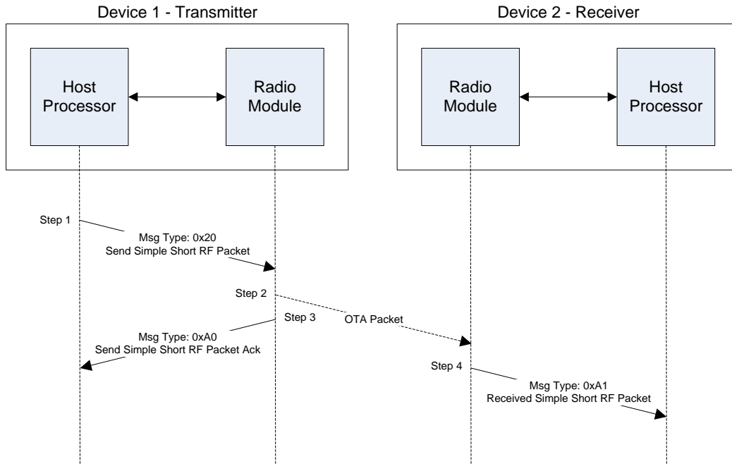
Figure 10 Send/Receive RF Message without RF Acks
